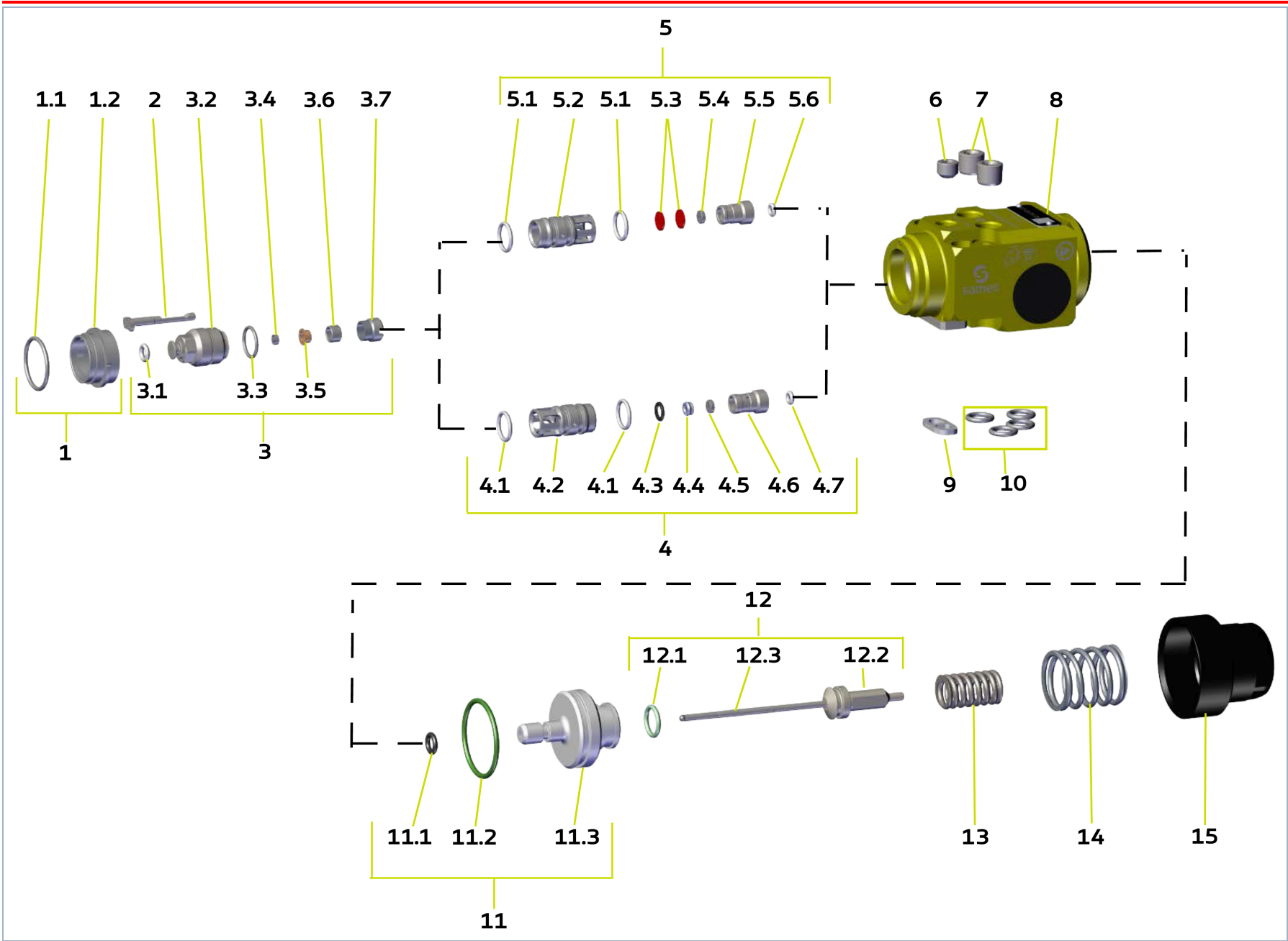
Gun shown without base, air cap, tip and fittings. Callout numbers match the parts list. Cartridge 4 = GT version; cartridge 5 = Rulon version. "-" = not sold separately.
